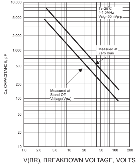
FIG.4-TYPICAL JUNCTION CAPACITANCE
